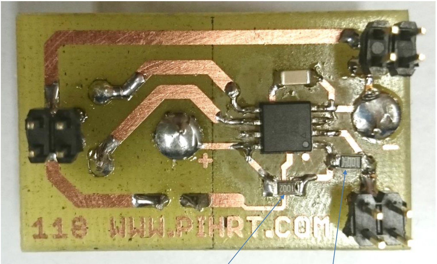
Rezistor 1002 (10k)
